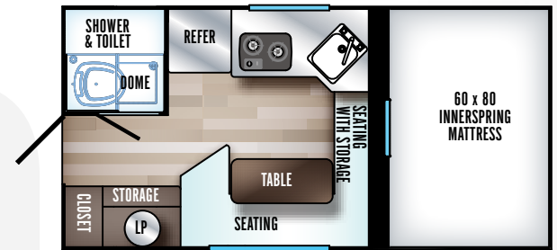
FULL SIZE TRUCK W/ 8' BED
