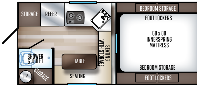
1/2 TON 6'6" BED W/OVERHANG
