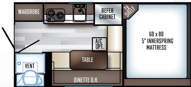
3/4 TON TRUCK W/ 6' 6" OR 8' BED
